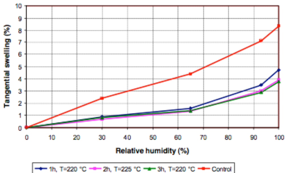
TANGENTIAL SWELLING, SPRUCE
