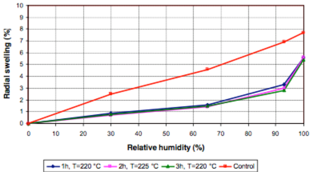
RADIAL SWELLING, SPRUCE
